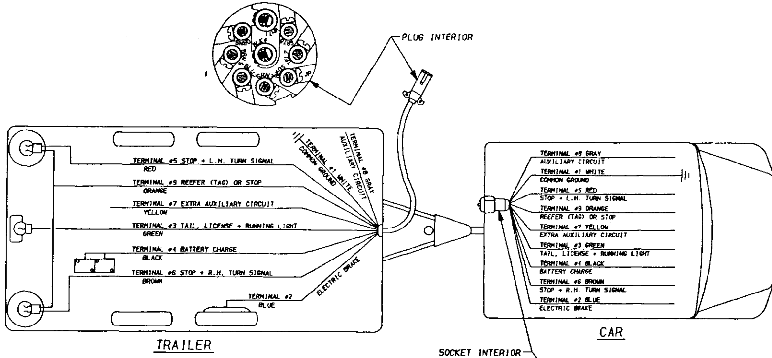
WIRE-UP SCHEMATIC - TRAILER TO CAR FOR NINE CIRCUIT CONNECTORS POLLAK NO. 12-905 SERIES CONNECTORS.
